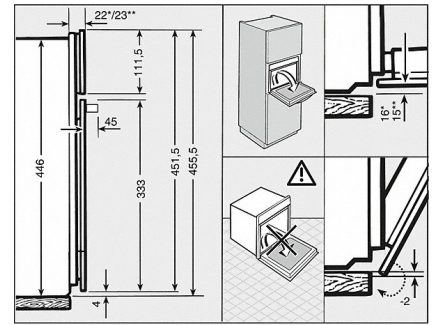
DG 6000 - Detalskiss ContourLine (skiss)
