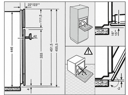
DG 6000 - Detalskiss ContourLine (skiss)
