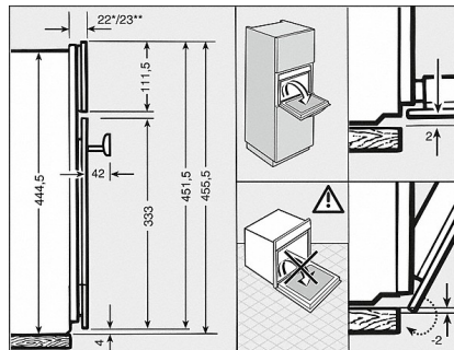
DGM 6000 PureLine (detalkjskiss)
