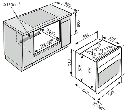
H 5000 EP/BP; H 6000 EP/BP; H 2000 EP/BP - 60 cm (skiss)
